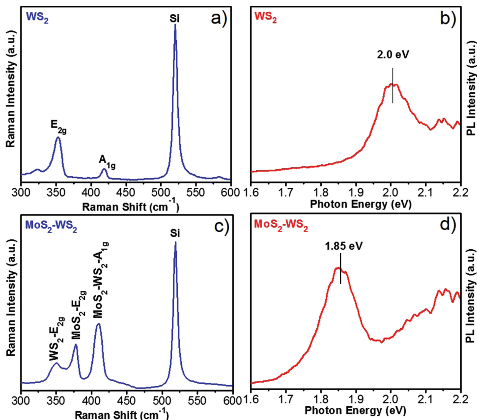
Figure 5. a,c) Raman and b,d) PL spectra of WS 2 and Mo x W 1-x S 2 film, respectively.
